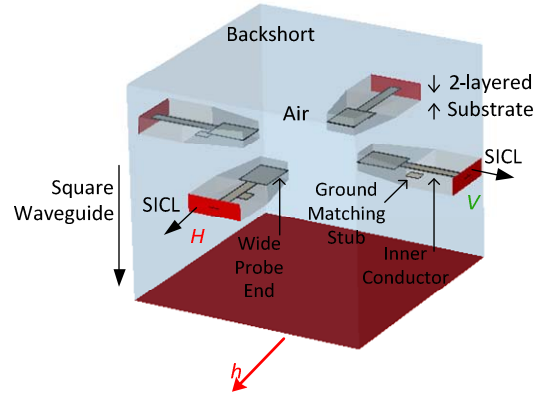
Fig. 2. Input short circuited square waveguide with SICL probes transversally placed in.
