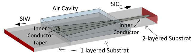
Fig. 3. Wideband double layer SICL to single layer SIW transition.
