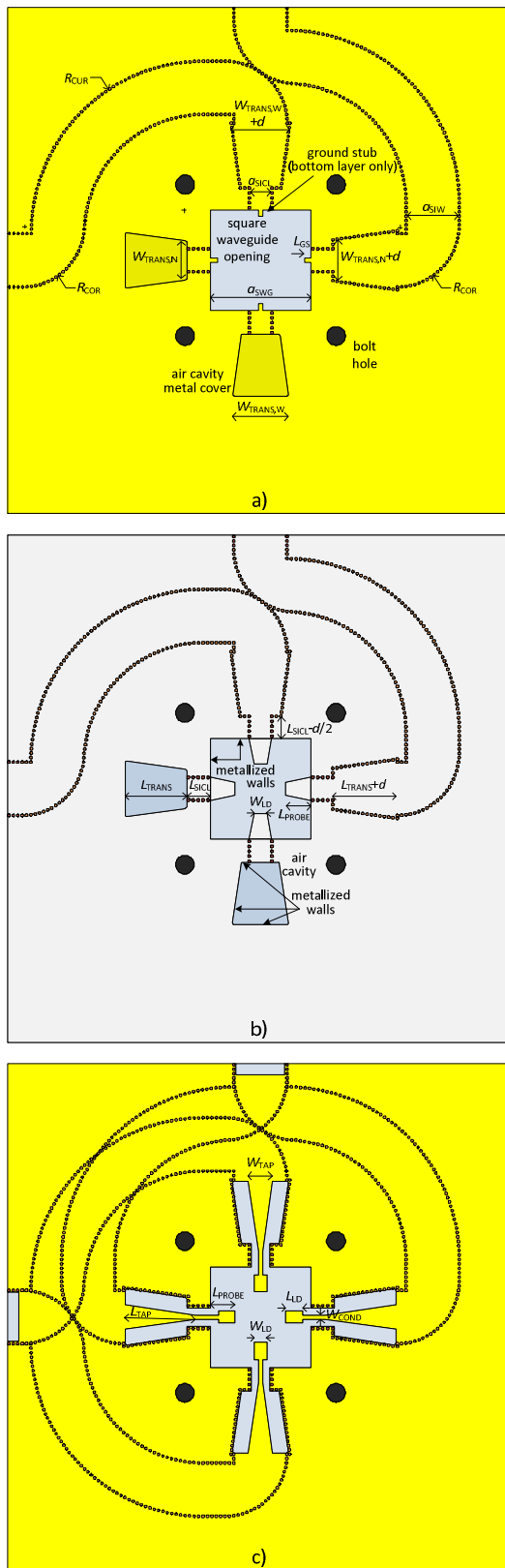
Fig. 5. PCB layouts of the wideband planar substrate integrated OMT: a) top/bottom metallization, b) top/bottom substrate and c) central metallization layer.
