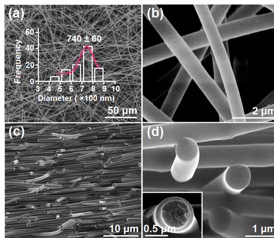
Figure 4. FESEM images of the tri-layer fibers: (a) and (b) Surface morphology and size distribution and (c) and (d) cross-sectional morphology. The lower left inset to (d) shows an occasional instance where different layers can be observed in the cross-section.
