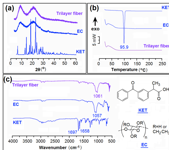
Figure 6. Characterization of the raw materials and the KET-loaded fibers: (a) XRD patterns, (b) DSC thermograms, and (c) IR spectra and chemical structures of KET and EC.
