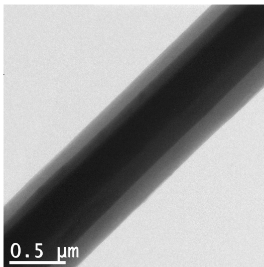
Figure 5. A TEM image of a tri-layer nanofiber.
