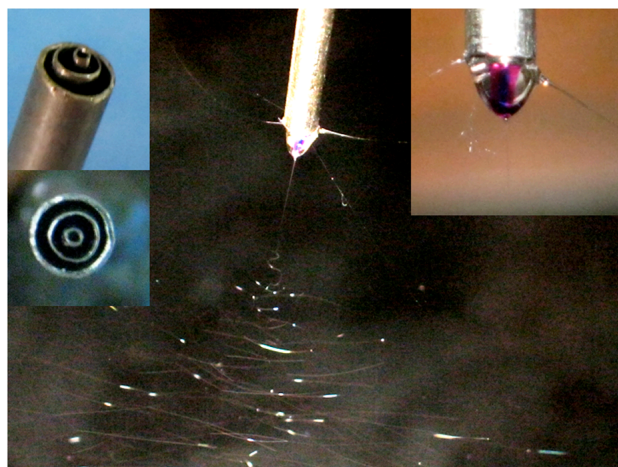
Figure 3. Digital photographs of the triaxial electrospinning process. The upper-left insets show the structure of the homemade spinneret, and the upper-right inset a typical compound Taylor cone.
