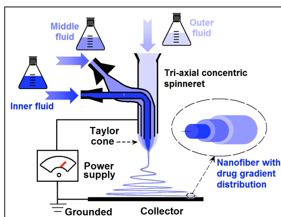
Figure 2. A schematic of the triaxial electrospinning process.
