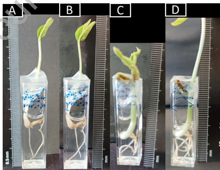
Figure 6 – Single mung bean plants grown for 16 (A, B) and 11 (C, D) days then placed into the dark chamber. Images show before (A, C) and after (B, D) measurement. The growth from A – B showed little change, however C-D showed an increased
