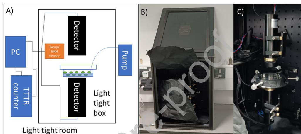
Figure 1 – Set up for photon emission detection in petri dish configuration. A) Schematic of the apparatus: two PMT detectors were orientated above and below the sample. A syringe pump remotely added water or solutions with dissolved chemicals mid-way through the experiment. A temperature and humidity sensor verified the experimental conditions. The detector TTL pulses were measured on a time-tagged time-resolved counter and recorded on a PC. B) Image of the apparatus inside the box: aluminium foil minimizes any accidental exposure to light when open and the lid features a foam seal. C) A close image of the dual photon counting units with an empty petri dish, the temperature and humidity sensor can be seen behind the dish. Further details of the dish and cuvette setup can be found in the Supporting Information.
