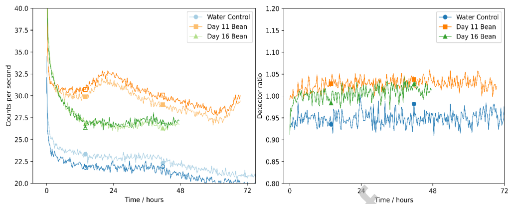
Figure 5 – (left) Single mung bean measured emission from two equi-distant detectors (left detector: dark, open symbols and right detector: light, closed symbols) of 3 samples: a 16-day grown bean (green triangles); an 11-day grown bean (orange squares); and a water-only blank (blue circles). DL in plant and water show decay whereas UPE shows increase in emission signal. (right) The difference in intensity of the detectors expressed as a ratio. This is due to the plant being positioned closer towards one side of the cuvette, as can be seen from the ratio remaining the same over the course of the experiment.
