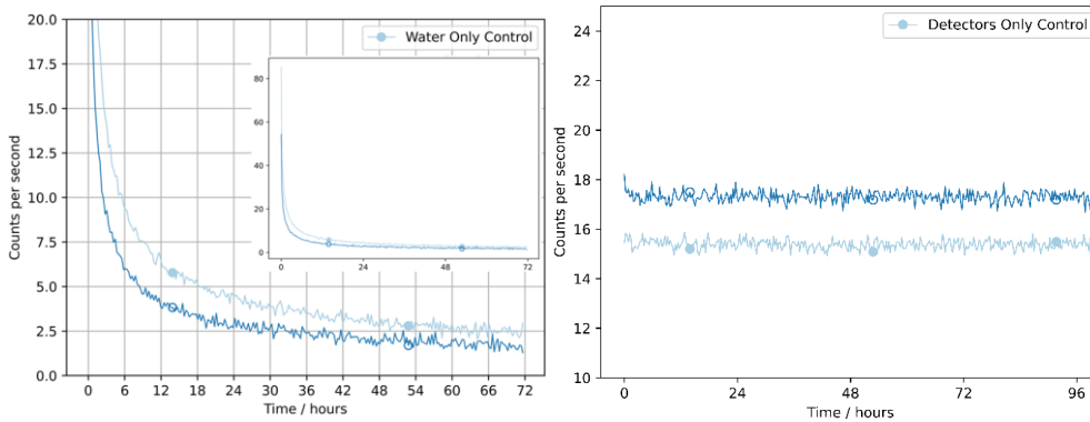
Figure 2 - (left) DL over time in a dish containing only water, with full measurement in inset. (right) Detectors in an empty chamber showing an average dark count of 15.4 and 17.3 cps over 4 days. Dark lines, open circles are detector below and light lines, closed circle are detector above.
