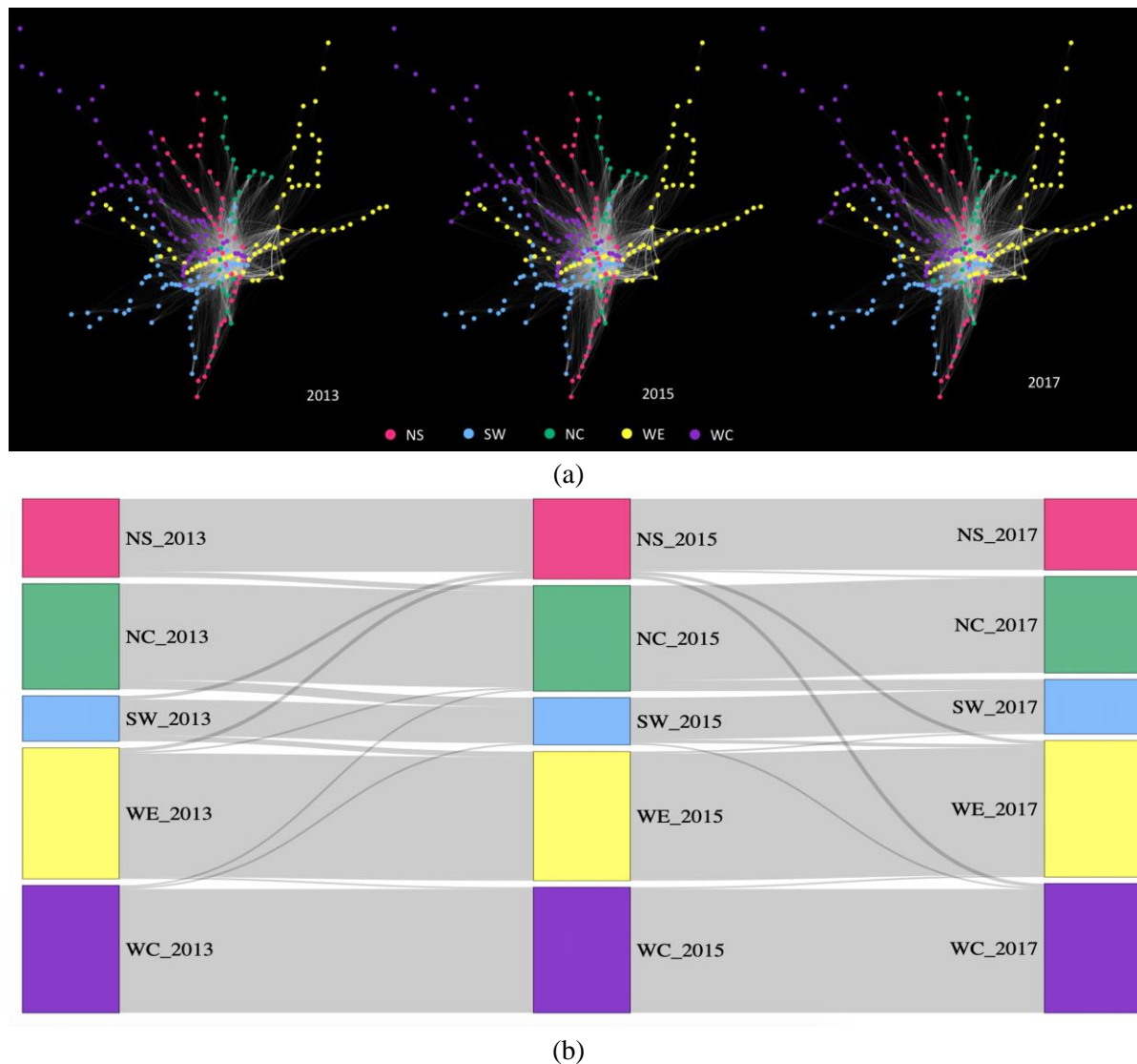
Fig. 4. The changing structure of Greater London in 2013, 2015 and 2017. (a) Community memberships of transit stations; (b) Sankey diagram of structural change.
