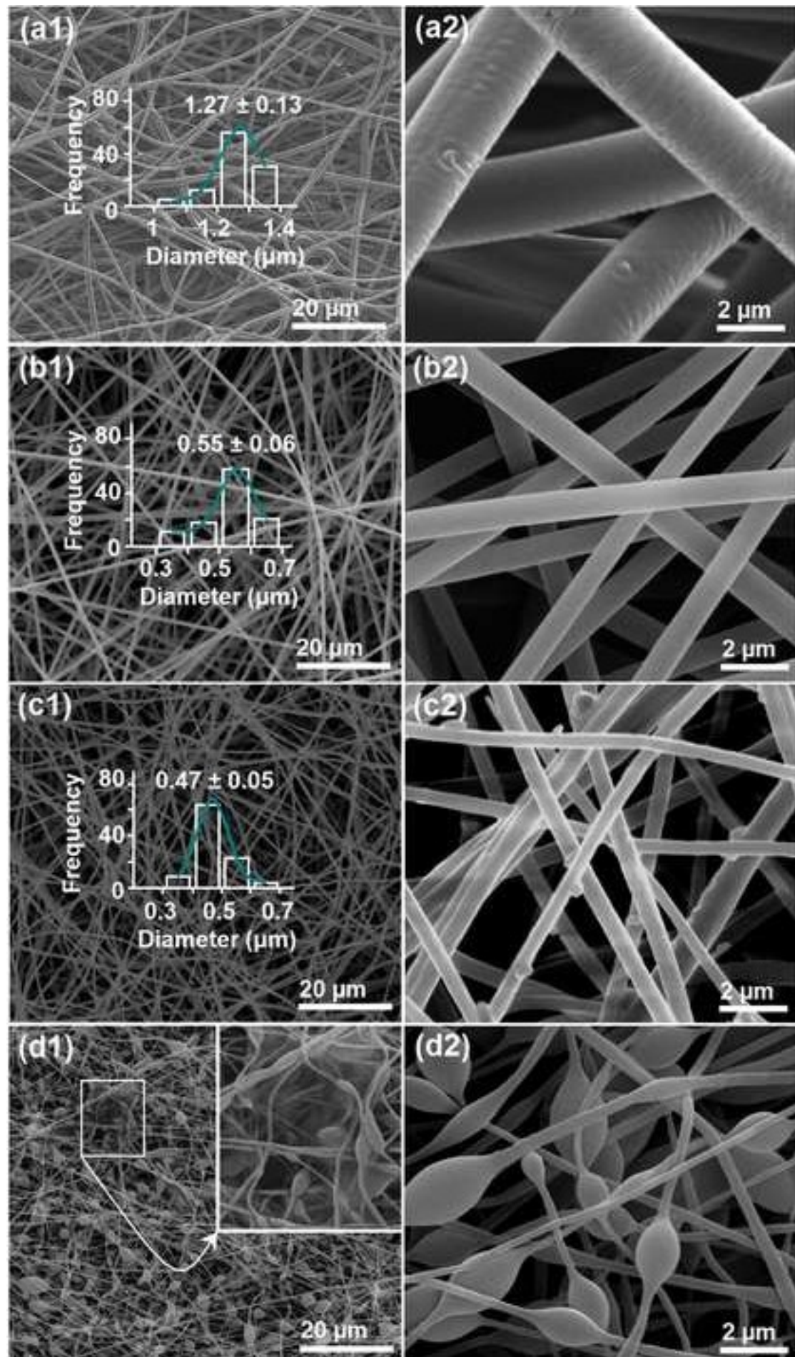
Fig.3 FESEM images of the core-shell nanofibers and their size Click here to do """"loajhigh resolution image
