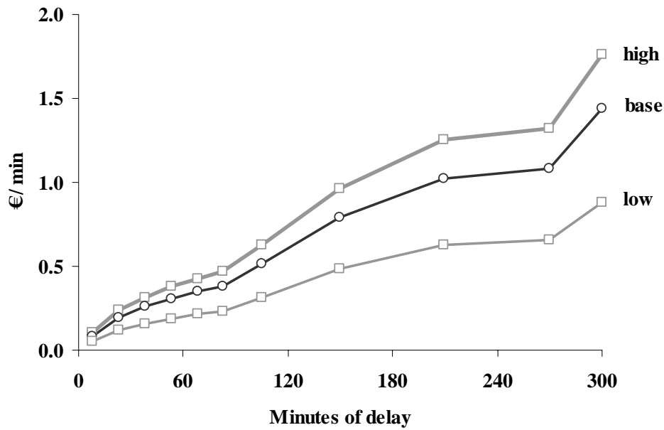
Figure 6. Passenger hard cost model by delay duration
