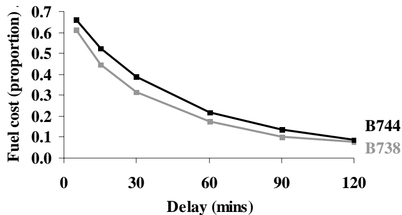
Figure 13. Proportional fuel cost as a function of delay duration
