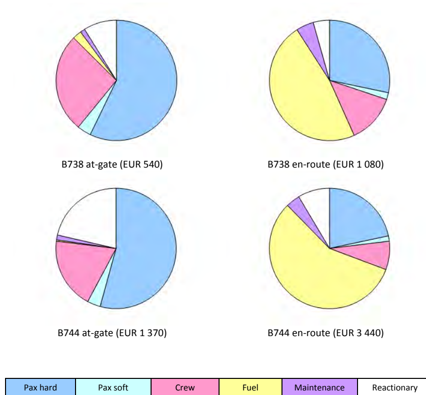
Figure 12. Example cost distributions for 15 min delays for B738 and B744
