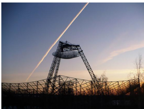
Fig. 5. Kharkiv incoherent scatter radar (on the left) and location of the instrumentation involved in the analysis (on the right).
