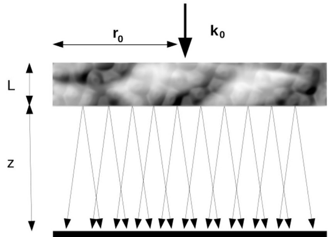
Fig. 15. Illustration of the scattering by a screen. From Grzesiak et al. (2022).
