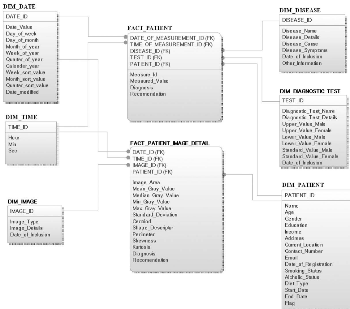
Figure 2. Logical representation of clinical dimensional model (logical data model for the clinical data mart)
