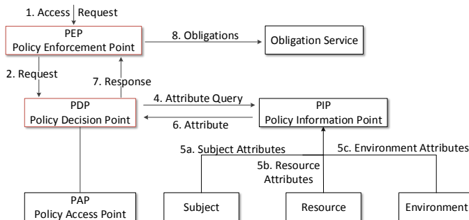
Figure 1: High level view of XACML Components
