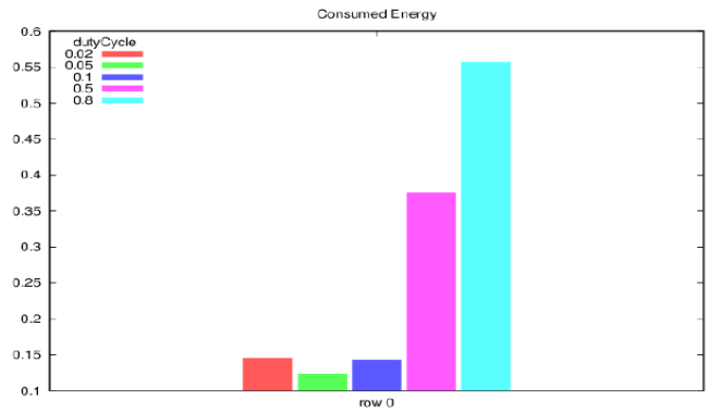
Fig. 2. Energy consumption based on duty cycles.
