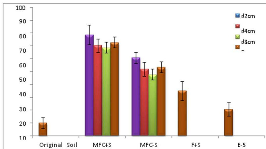
Figure 5. Percentage total COD (TCOD) removal at different distances from the anode for the active MFCs and control reactors at the end of 60 days of MFC operation at ambient temperature. R_{avg} is the average of removal efficiencies at different radial distance from the anode. Values are means of triplicate measurements \pm SD. E-S and F+S mean controls without and with surfactant addition respectively.
