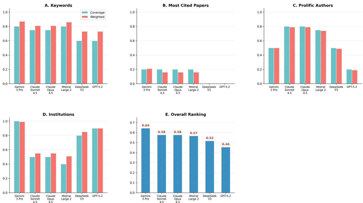
Fig 2. Benchmark Performance of Six Frontier LLMs on UK Biobank Knowledge Retrieval Tasks (January 2026). (A) Keywords: Keyword recognition benchmark comparing Coverage Score (proportion of top 20 keywords matched) and Weighted Coverage Score (frequency-weighted) across all six models. Gemini 3 Pro and Mistral Large 2 achieved highest coverage (0.80), followed by Claude models (0.75). GPT-5.2 and DeepSeek V3 scored 0.60. (B) Most Cited Papers: All models struggled with this challenging task. Gemini 3 Pro scored highest (Coverage 0.20, Weighted 0.21), while GPT-5.2 and DeepSeek V3 failed to identify any matching papers (0.00). (C) Most Prolific Authors: Each model's output is assessed for matching the top 20 authors by publication count. Coverage Scores capture how many authors each LLM mentions, while Weighted Coverage Scores emphasize authors with more total publications. (D) Applicant Institutions: Shows performance in detecting the 10 most frequent UK Biobank applicant institutions. Scores are weighted according to the institution's application counts. (E) Overall Ranking: Overall weighted coverage ranking across all four tasks. Gemini 3 Pro leads (0.643), followed by Claude Sonnet 4.5 and Claude Opus 4.5 (0.577 each), Mistral Large 2 (0.567), DeepSeek V3 (0.517), and GPT-5.2 (0.455).
