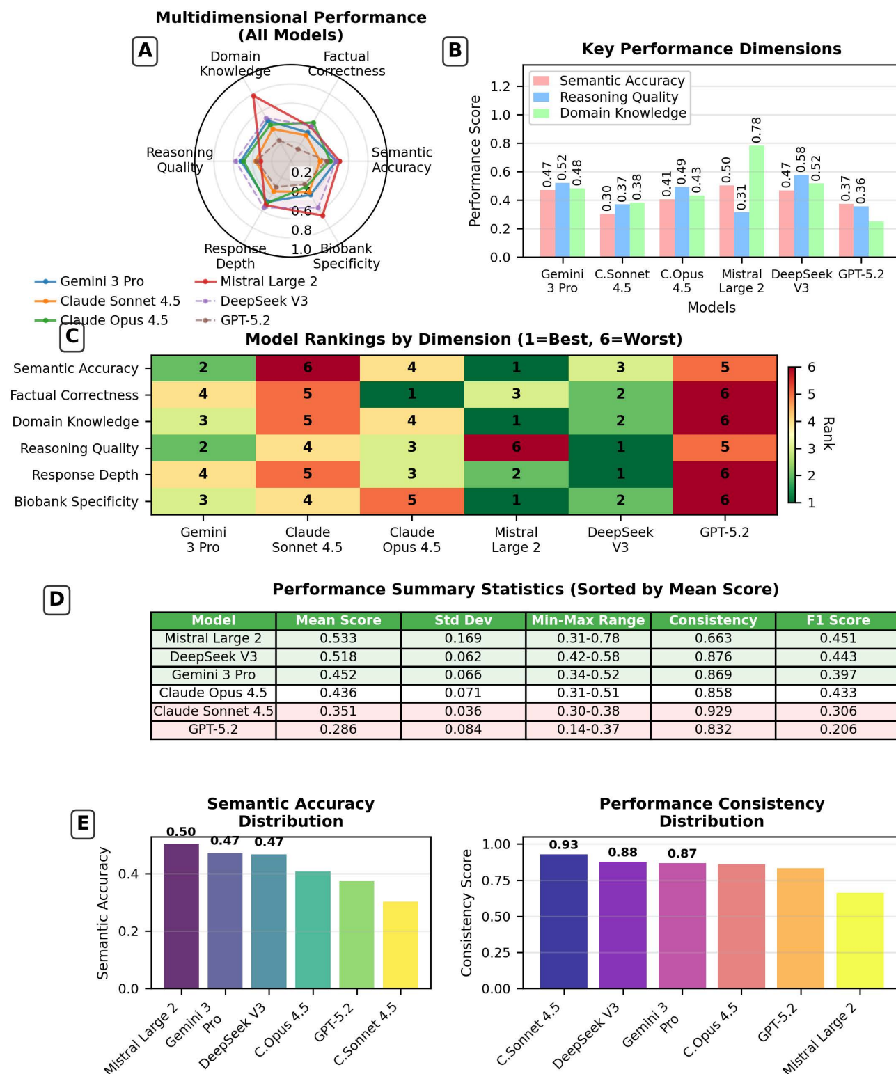
Fig 3. Multidimensional Performance Analysis of Six Frontier Large Language Models on UK Biobank Benchmark (January 2026). (A) Radar plot showing normalised scores (0–1 scale) across six evaluation dimensions for all six models. Each axis represents one dimension: Semantic
