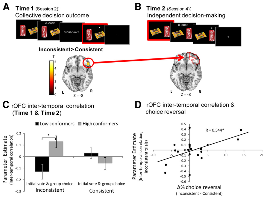
Figure 3. OFC response to a collective decision predicts subsequent response when making an individual choice. A , Enhanced BOLD response was observed in the right OFC when subjects learn that the collective decision was inconsistent with their own vote, relative to when it was consistent ( p < 0.05 FWE, anatomical SVC; displayed at p < 0.005 , uncorrected). B , BOLD signal was extracted from this region for each specific trial and added as a parametric modulator predicting BOLD signal when an individual decision was to be made regarding the same pair at a later time. Parameter estimates were then averaged over the anatomically defined subregions of the right OFC as defined by the AAL atlas. For illustration purposes, the red frames in the trial design in A and B denotes the time of the trial when BOLD response was analyzed. C , A significant interaction emerged in the right superior OFC. Past OFC response to collective decision positively predicted subsequent OFC signal when making an individual selection between a pair of items for which subjects' initial vote was inconsistent with the collective decision in high conformers, a trend for a negative correlation emerged for low conformers, and no correlation emerged when the initial vote was consistent with group outcome. D , Across participants, the relationship between past and subsequent OFC response predicted behavioral change (i.e., choice reversals). Specifically, the greater the positive correlation between these signals on inconsistent trials, the more likely an individual was to reverse their choices to align with collective decisions that were initially inconsistent with their own. *p < 0.05 , two-tailed t test; error bars indicate SEM.
