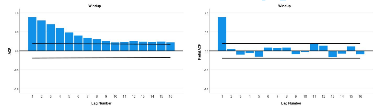
Figure 3 ACF & PACF of Dependent Variable
