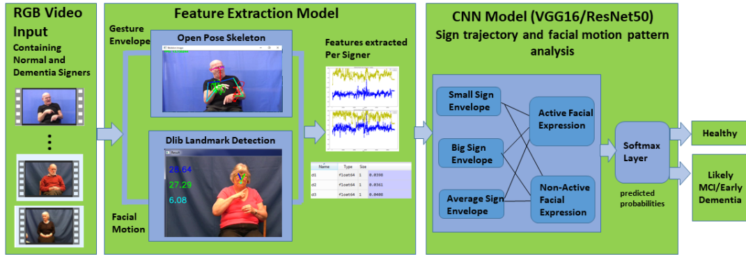
Figure 1: The Proposed Pipeline for Dementia Screening
