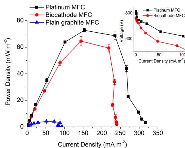
Fig 2. Maximum power density for each cathode catalysts in MFC measured using polarization tests as in Mani and colleagues (2019). Inset: Voltage/current graph for the cathodes indicating the losses.
