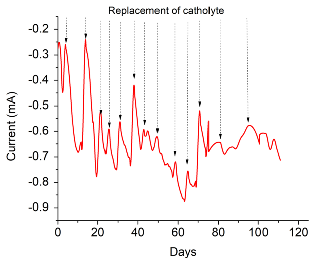
Fig 1. Chronoamperometry of biofilm showing the peak current for each cycle observed through half-cell microbial enrichment method (Refer Supplementary S1).
