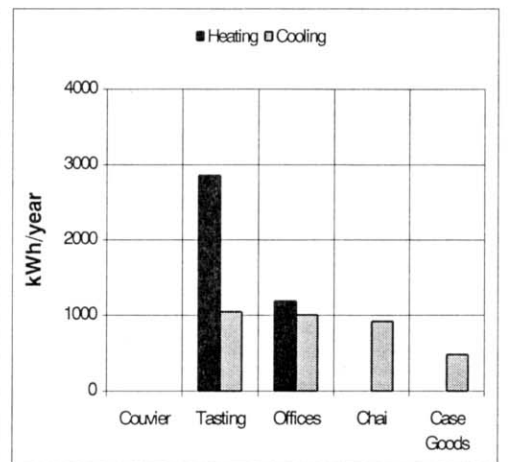
Fig. 5 – Annual Energy Consumption in the Reference Building
