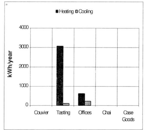
Fig. 3 – Annual Energy Consumption in the Proposed Building
