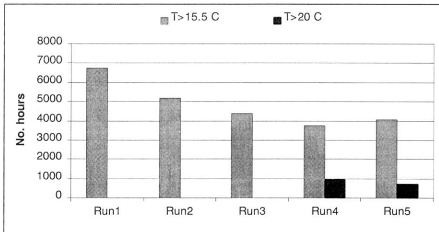
Fig. 4 – Annual Predicted Temperatures in Barrel Room
