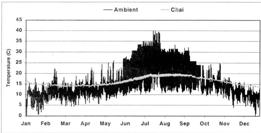
Fig. 2 – Annual Predicted Temperatures in Barrel Room
