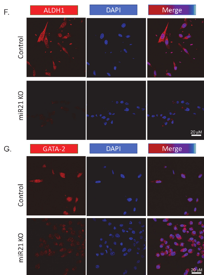
Figure 5. The silencing of miR-21 reduced the mesenchymal phenotype of MDA-MB-231 cells. (A) Protein levels of epithelial and mesenchymal markers were tested by Western blotting. \beta -actin was used as a loading control. The densitometry graph represents protein expression levels of band intensities obtained from at least three independent experiments. The relative band intensities of each sample were calculated by normalizing against \beta -actin. Each data point represents average \pm SD. **** p < 0.0001 . ( n = 3 ) (B–E). Immunofluorescence assay was performed to show E-cadherin levels and localization, Snail, Zeb-1, and vimentin (green). (F–G) Cancer stem cell markers ALDH1, GATA2 expressions (red), and localizations were assessed by using immunofluorescence in MDA-MB-231 wt and miR-21 KO cells. ToPro3 (blue) was used for nuclei. KO2 immunofluorescence results were shown as a representative to compare to wt ( n = 3 ), scale bar 20 nm.
