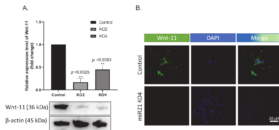
Figure 6. miR-21 deletion downregulated Wnt-11 expression in MDA-MB-231 cells. (A) The Wnt-11 expression was examined by Western blot analysis in MDA-MB-231 wt and two selected colonies for miR-21 KO cells. \beta -actin was used as a loading control. The densitometry graph represents protein expression levels of band intensities obtained from at least three independent experiments. The relative band intensities of each sample were calculated by normalizing against \beta -actin. Each data point represents average \pm SD. ** p < 0.01 . ( n = 3 ) (B) The Wnt-11 expression was examined by immunofluorescence, and ToPro3 (blue) was used for nuclei. Clone 2 (KO2) immunofluorescence results were shown as a representative to compare to wt ( n = 3 ), scale bar 20 \mu m.
